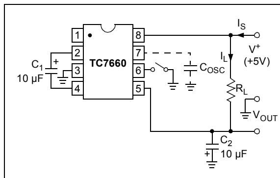
FIGURE 1-1: TC7660 Test Circuit.
