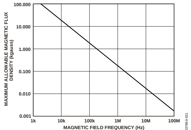
Figure 19. Maximum Allowable External Magnetic Flux Density
